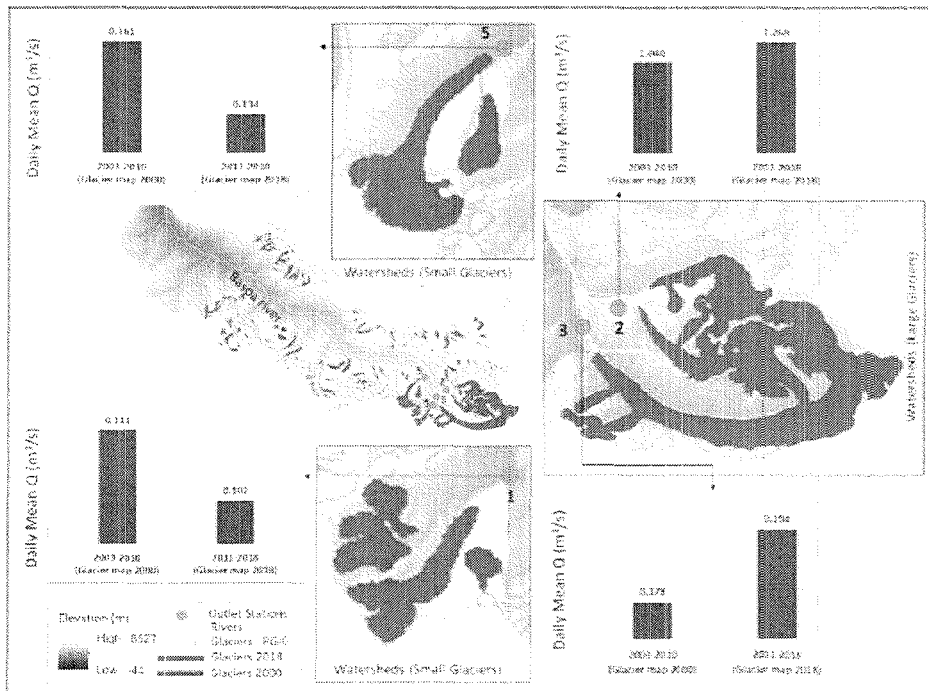
Figure 20: Glacier area and glacier melt runoff (glacier Q, daily mean in m^3/s ) changes as per selected watersheds comprises with large size and small size glaciers in BRB.
