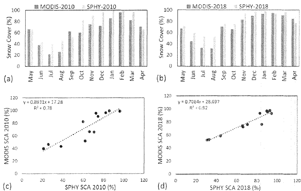
Figures 7: (a) time series plots between MODIS derived monthly SCAs during 2010, (b) time series plots between MODIS derived monthly SCAs during 2018, (c) regression plots showing comparison between observed snow and modelled snow-covered areas (%) during 2010, and (d) regression plots showing comparison between observed snow and modelled snow-covered areas (%) during 2018.
