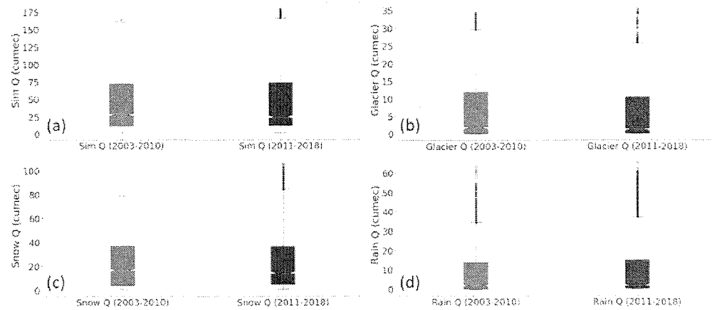
Figure 14: Variations in Sim Q (a), Glacier Q (b), Snow Q (c) and Rain Q (d) computed during two times i.e. 2003-2010 and 2011-2018.
