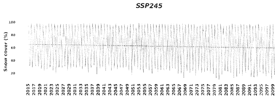
Figure 22: Shows the long-term change in snow cover (%) during 2015-2100 as per (CMIP6 Models) SSP245.
