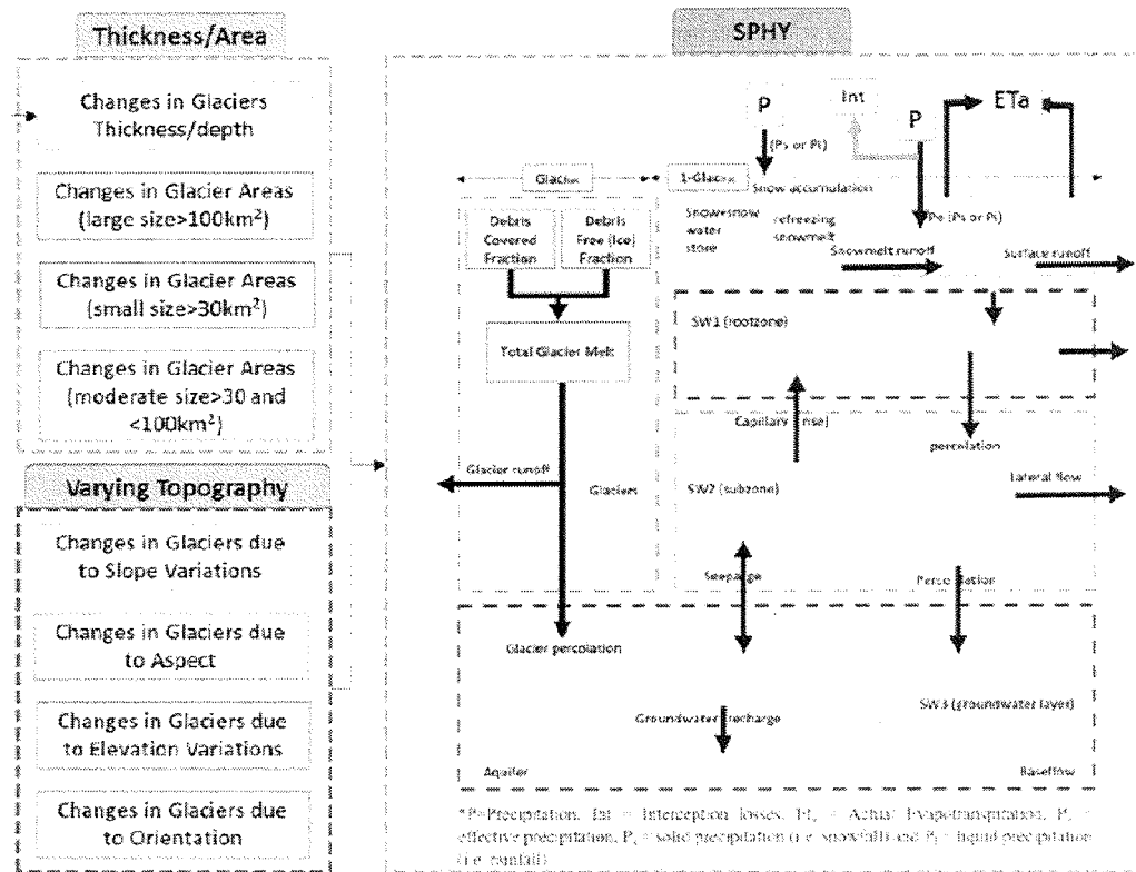
Figure 4: Schematic and methods of SPHY modeling framework.
