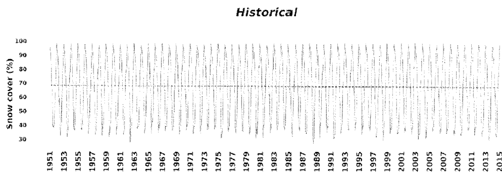
Figure 21: Shows the long-term change in snow cover (%) in the Historical time during 1951-2014.
