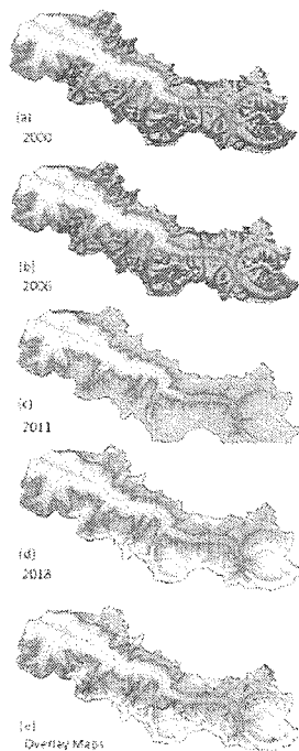
Figure 5: Temporal variations in glacier maps of Baspa basin highlighting reduction in the glacier area from 2000 to 2018: (a) 2000, (b) 2006, (c) 2011, (d) 2018 and (e) overlay of all year maps.
